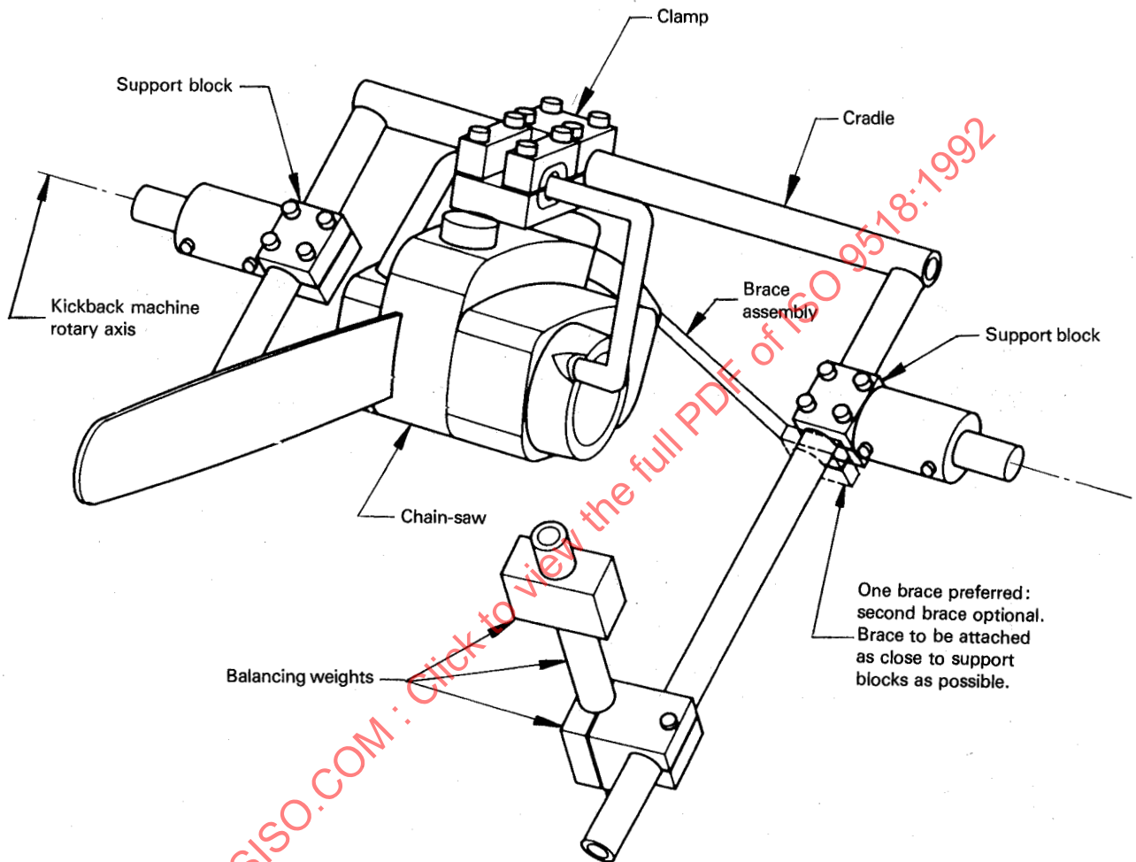
Figure 4 — Installation of saw/clamp/cradle assembly
