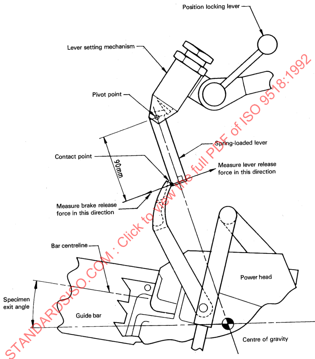
Figure 7 — Adjustment of chain brake actuator
