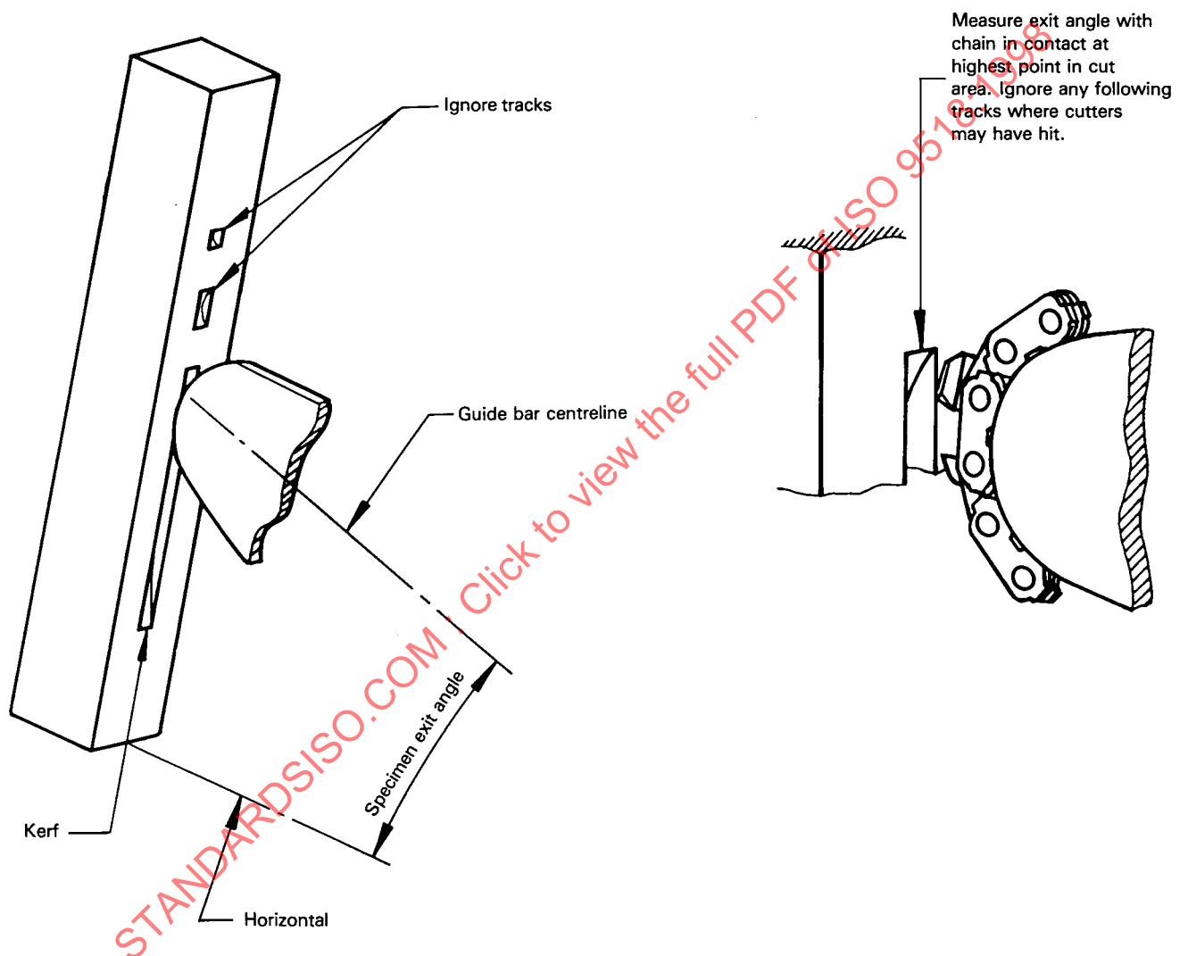
Figure 8 — Specimen exit angle measurement
