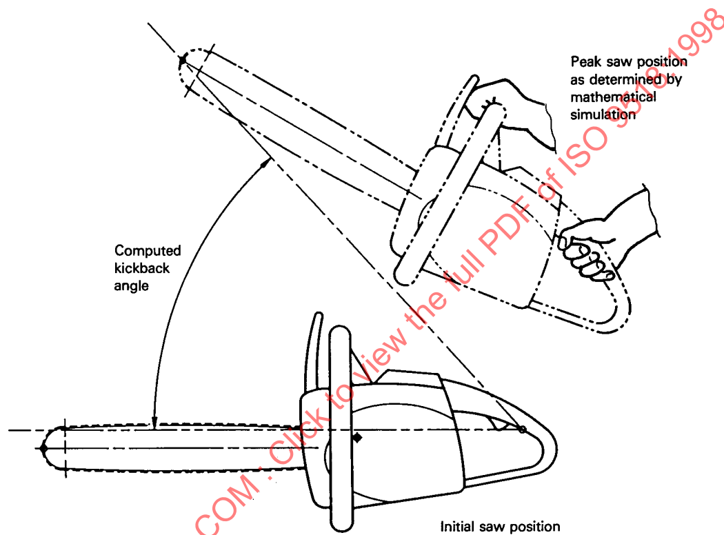
Figure 1 — Computed kickback angle
