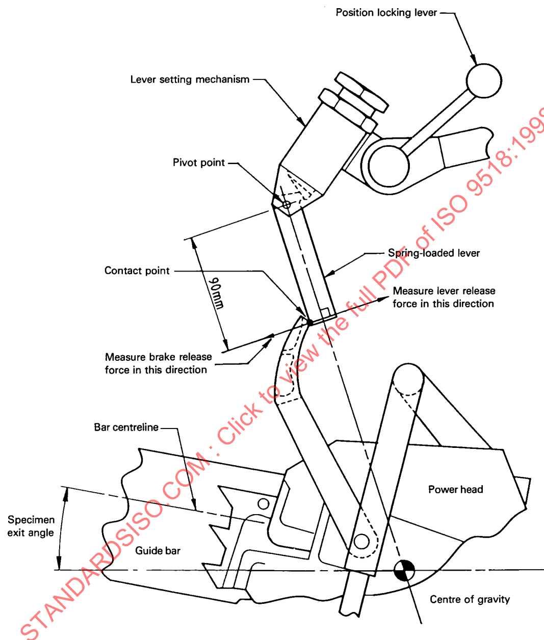
Figure 7 — Adjustment of chain brake actuator
