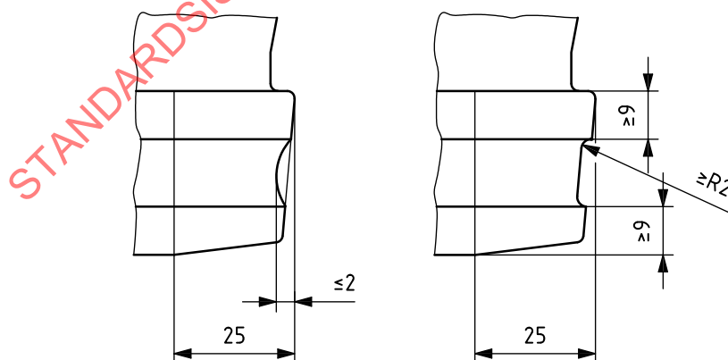
Figure 2 — Lateral grooves at heel
