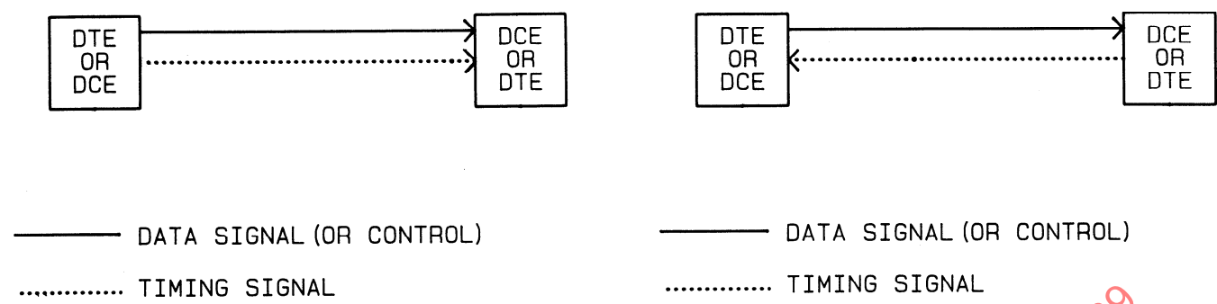
Figure 7 — Codirectional timing
