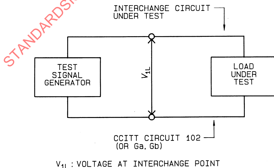
Figure 2 — Test arrangement for V.28 loads
