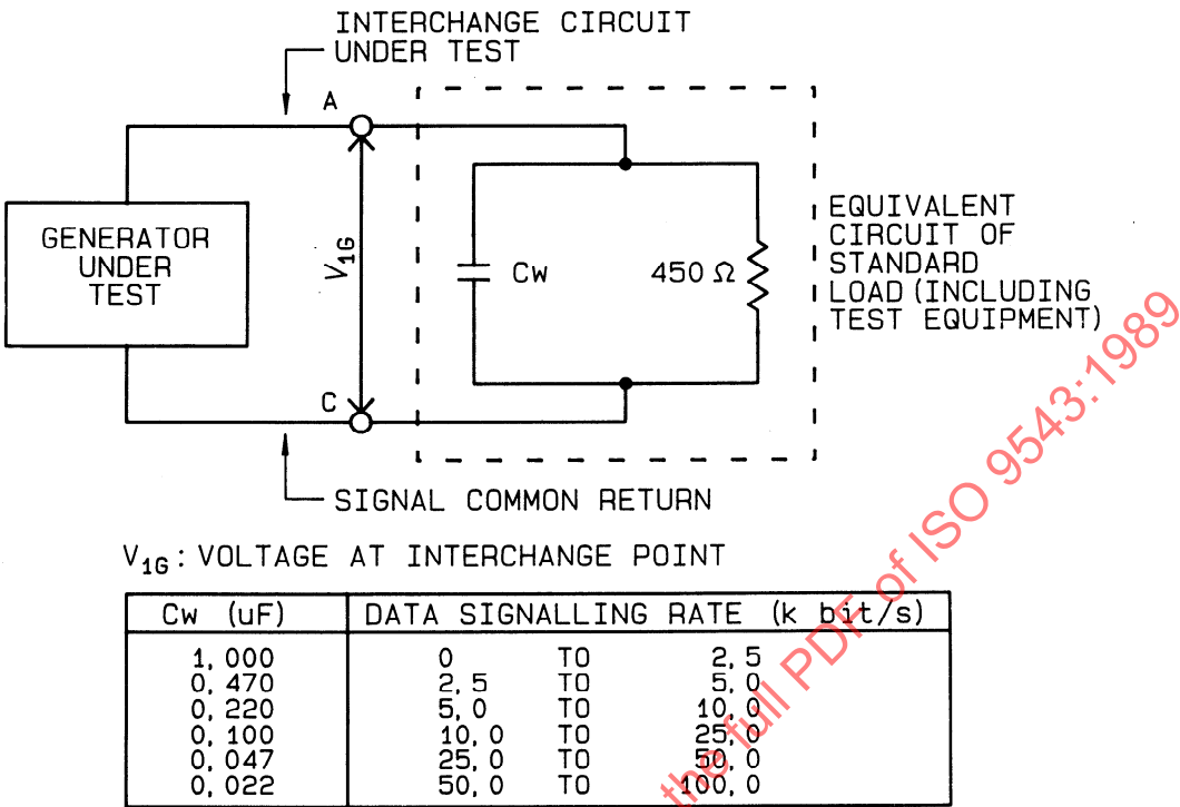
Figure 3 — Test arrangement for V 10 generators and values of C_w
