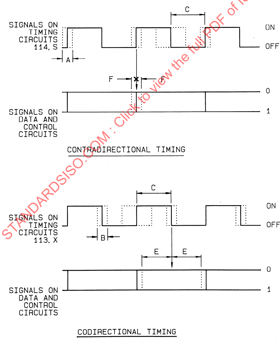
Figure 9 — Illustration of signal quality parameters on interchange circuits associated with the transmit direction
