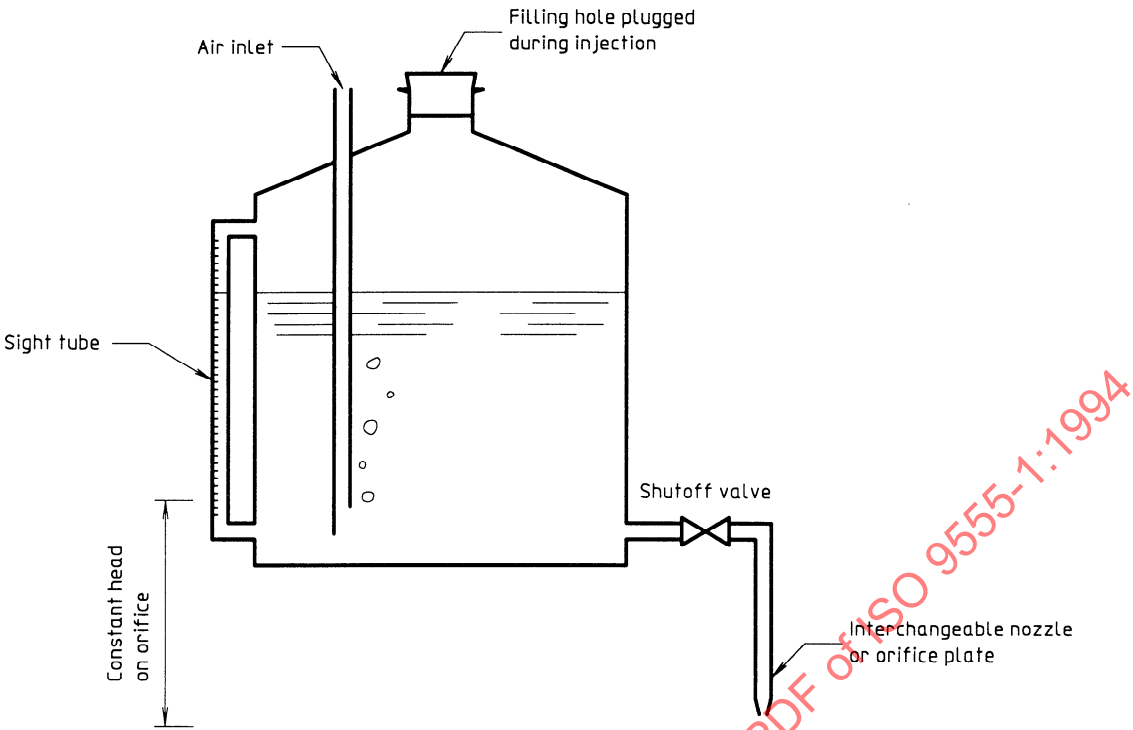
Figure 6 — Mariotte constant head vessel
