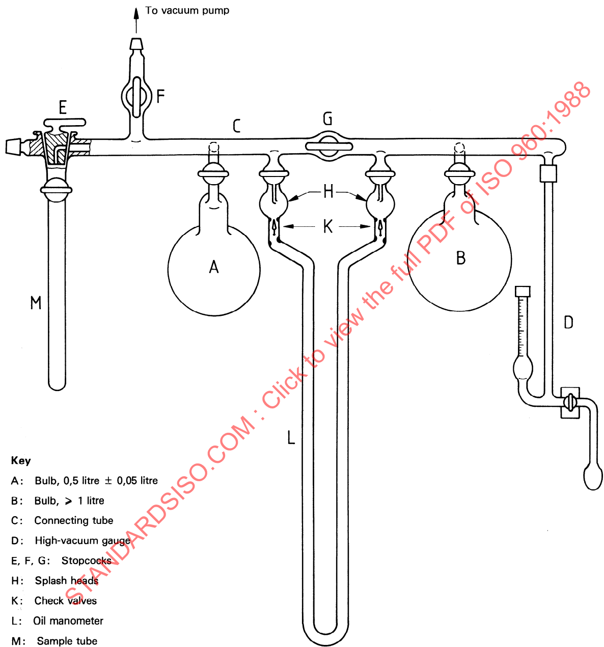
Figure 3 — Apparatus for determination of water content by method D (manometric)
