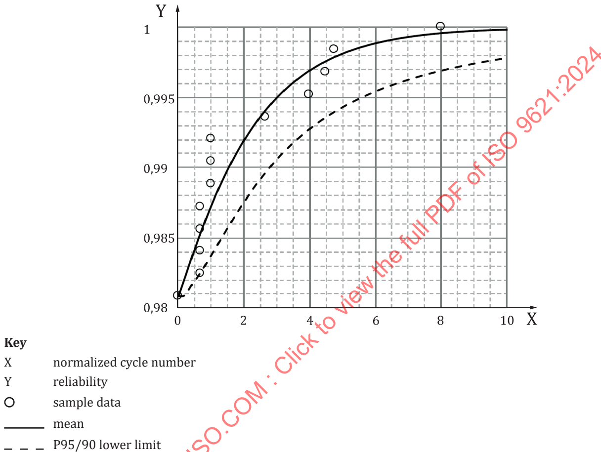
Figure B.2 — Relationship between reliability and normalized cycle number
