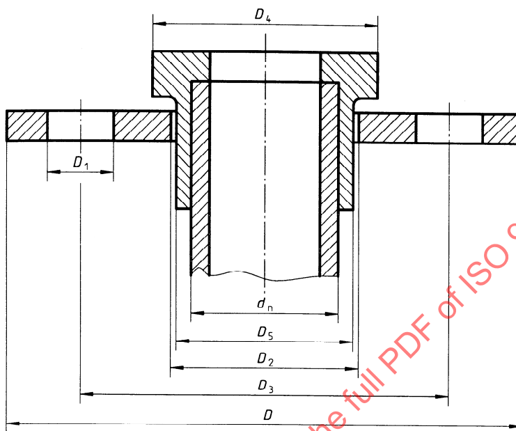
Figure 1 — Socket fusion and solvent-cemented systems
