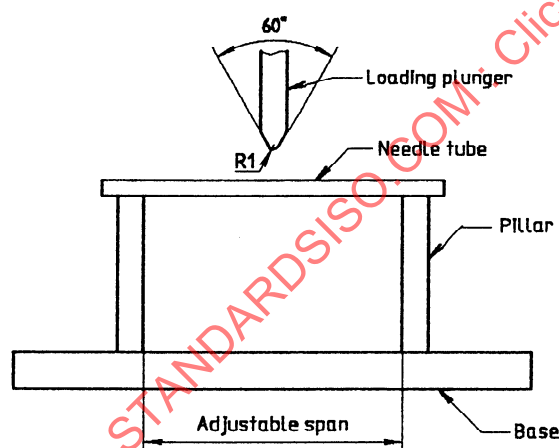
Figure C.1 — Apparatus for stiffness test
