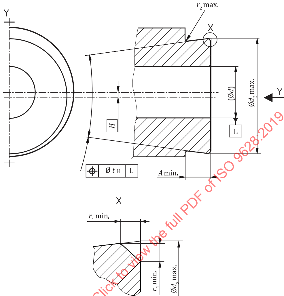
Figure 5 — Eccentric extension of inner ring
