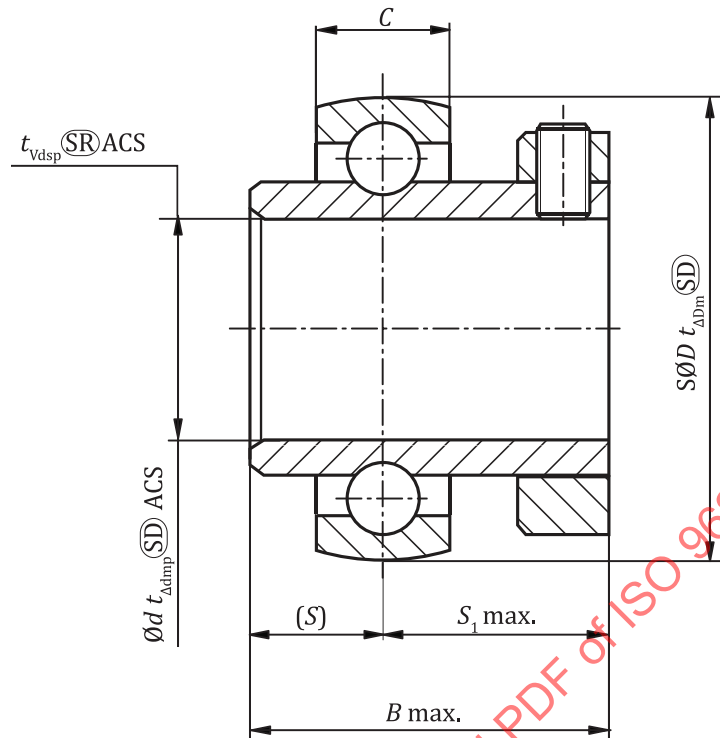
Figure 2 — Bearing with concentric locking collar around the inner ring — Intermediate overall width
