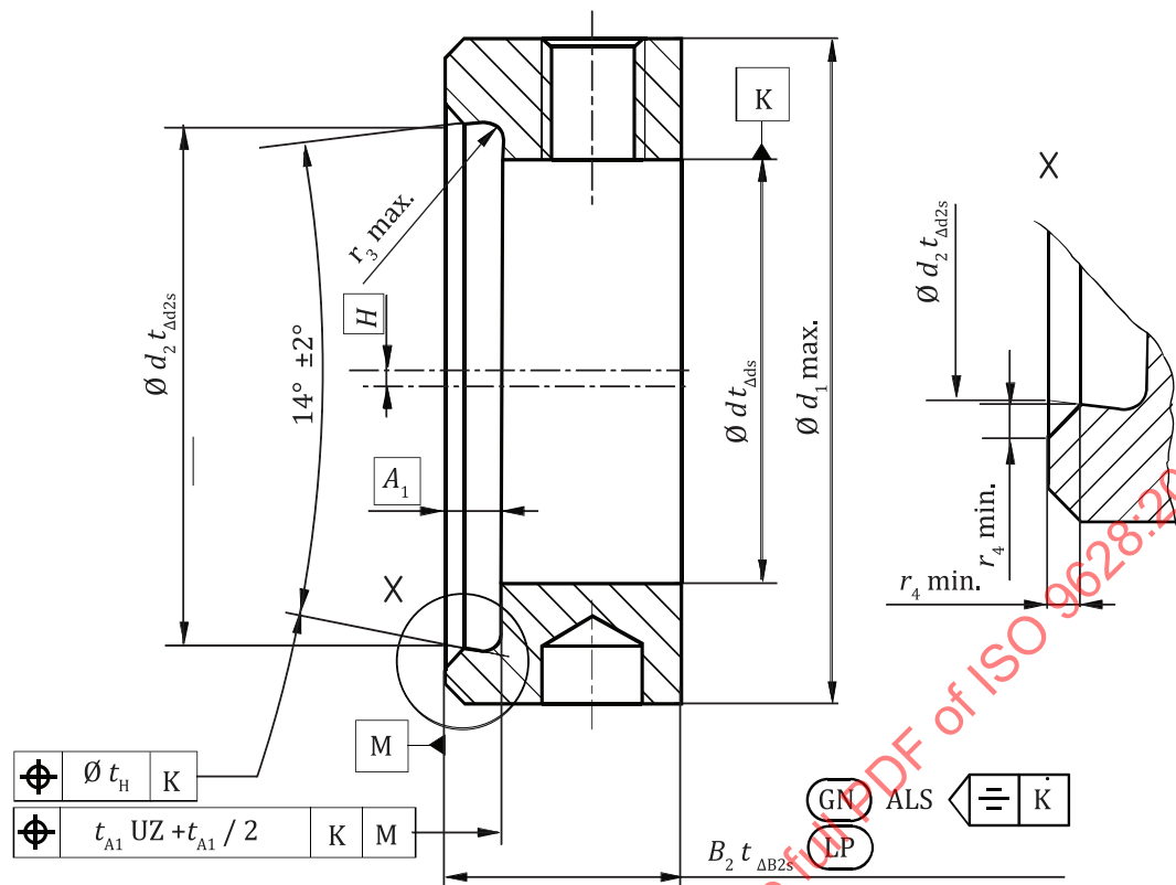
Figure 6 — Eccentric locking collar
