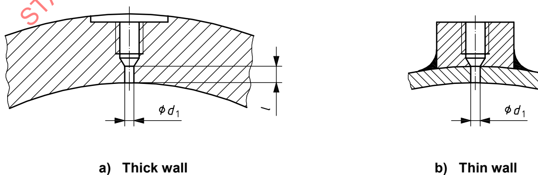
Figure 3 — Static pressure taps in thick and thin-wall piping
