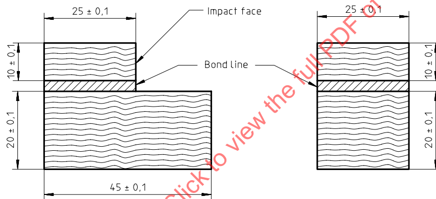
b) Wood-to-wood specimen showing grain direction
