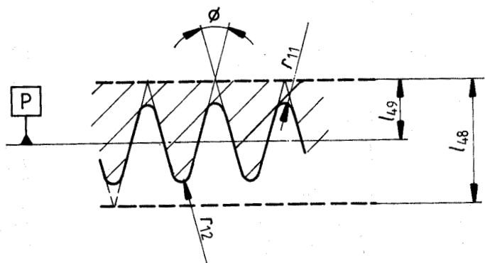
Figure 14 — Teeth of the toothed rim
