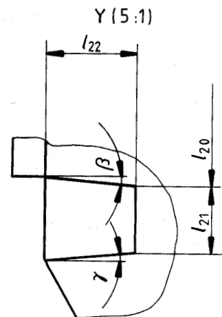
Figure 10 — Cross-section of a location notch
