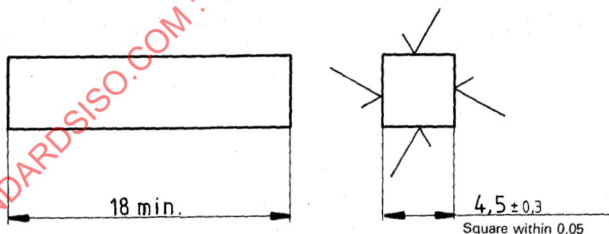
Figure C.1 — Ferrite wear bar
