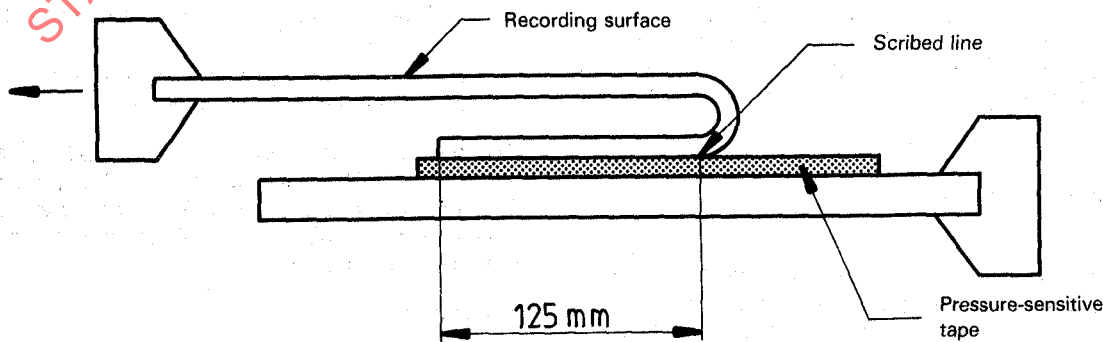
Figure 1 — Coating adhesion
