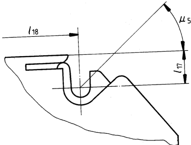
Figure 17 — Leader block in case
