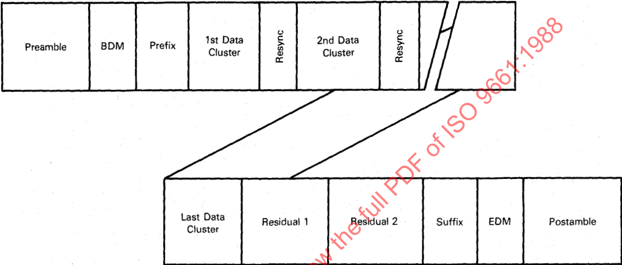
Figure 25 — Recorded Data Block
