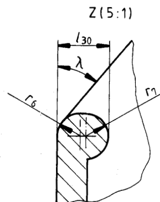
Figure 11 — Cross-section of a detail of the opening of case
