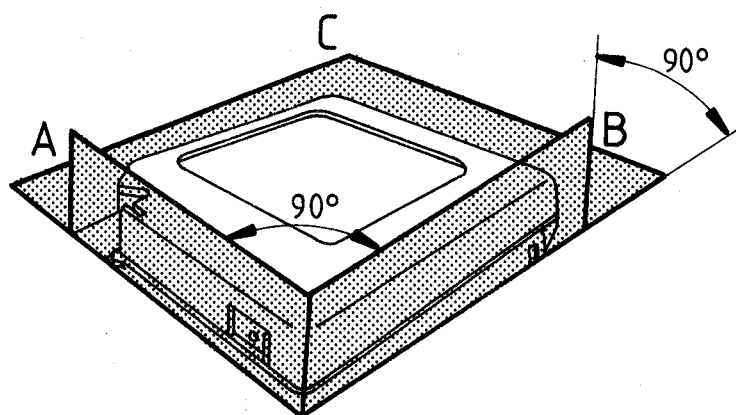
Figure 3 — Cartridge
