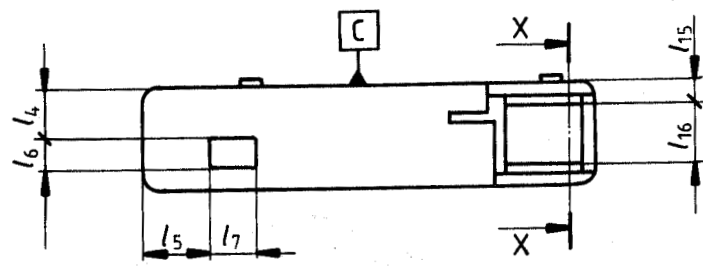
Figure 4 — Front side of case
