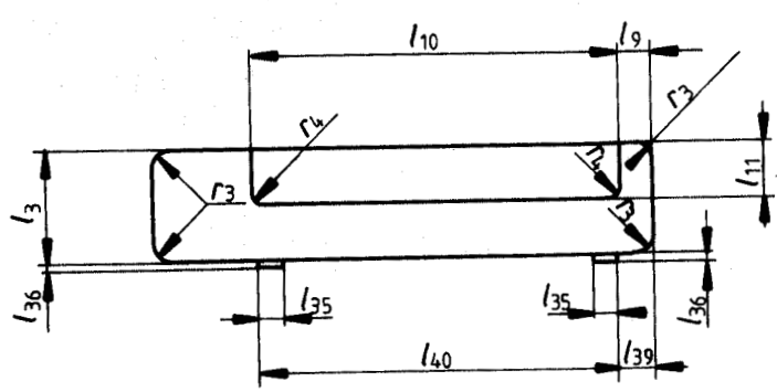
Figure 6 — Rear side of case
