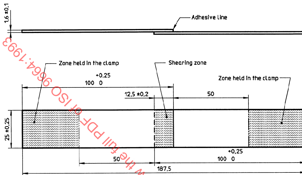
3 a) Steel substrates held in a clamp
