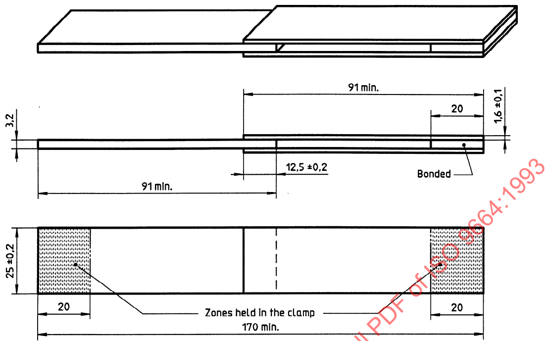
3 c) Aluminium substrates with double overlap
