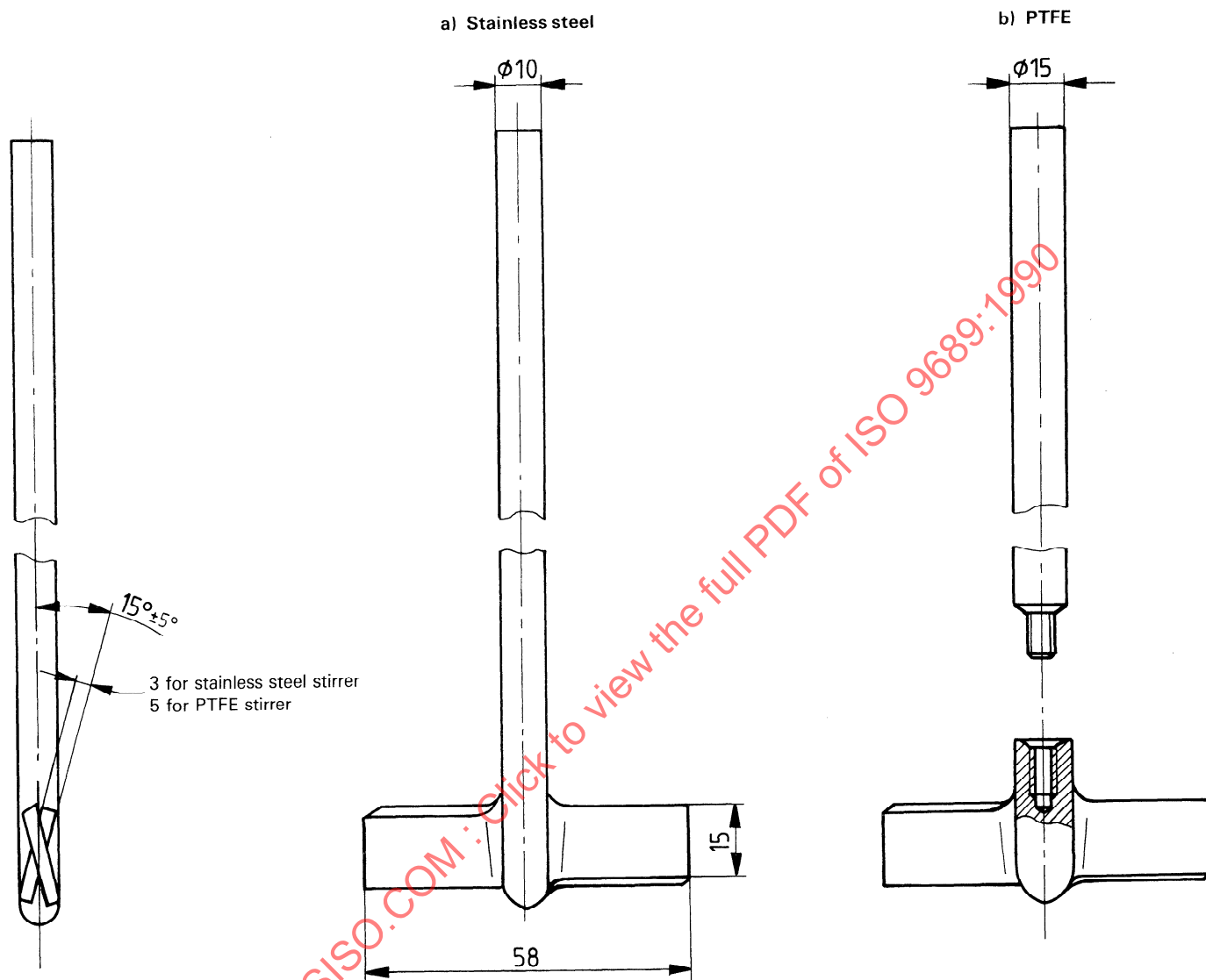
Figure 3 — Stirrers
