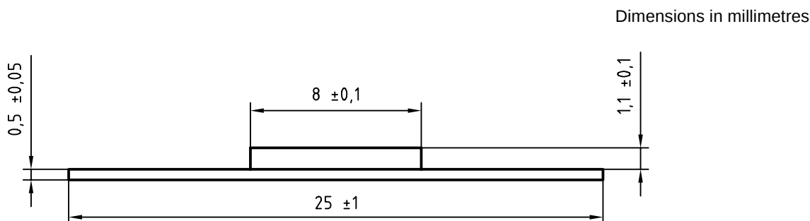
Figure 3 — Test specimen configuration
