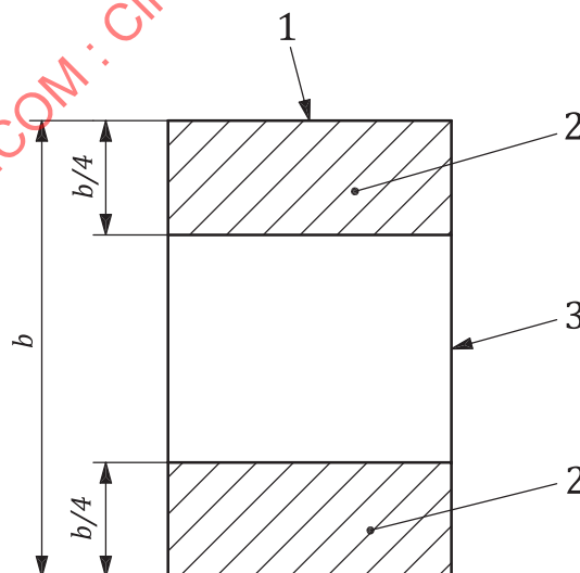
Figure A.1 — Illustration of knot projection area
