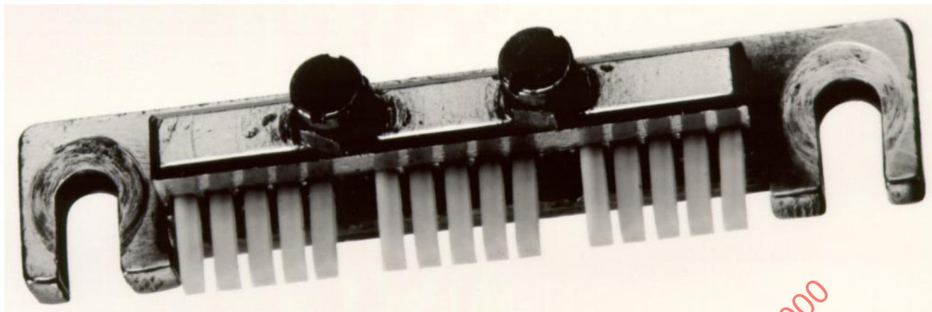
Figure 3 — Assembled clamp with test specimens
