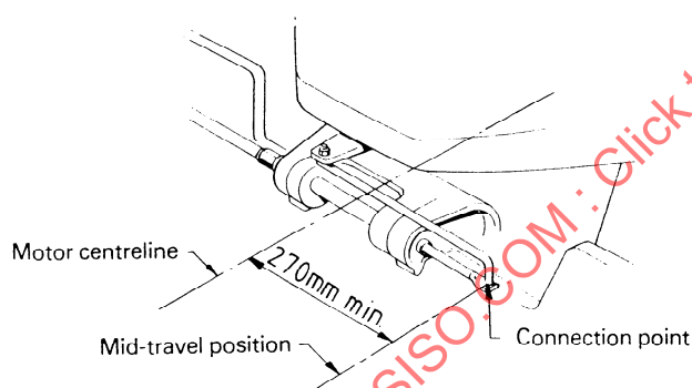
Figure 6 — Motor-mounted steering system
