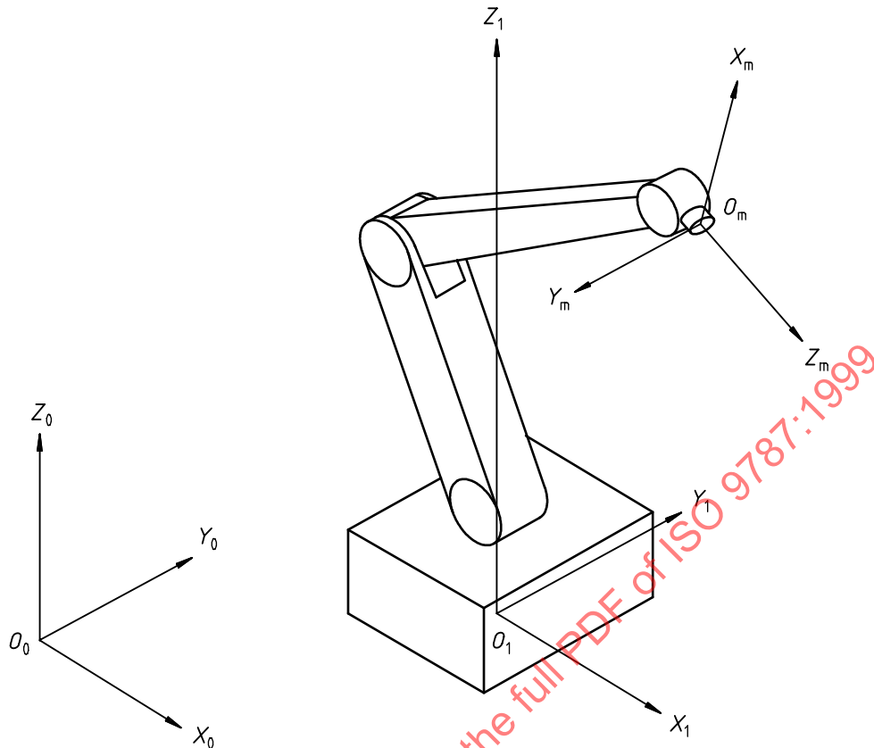
Figure 3 — Examples of coordinate systems
