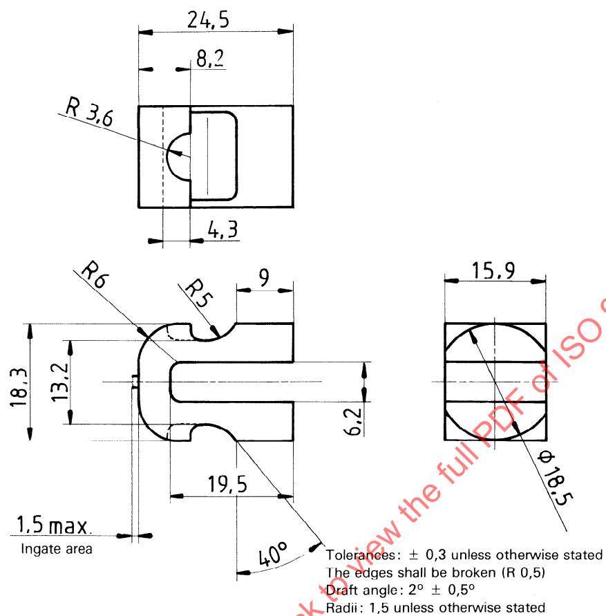
Figure 2 — Plunger
