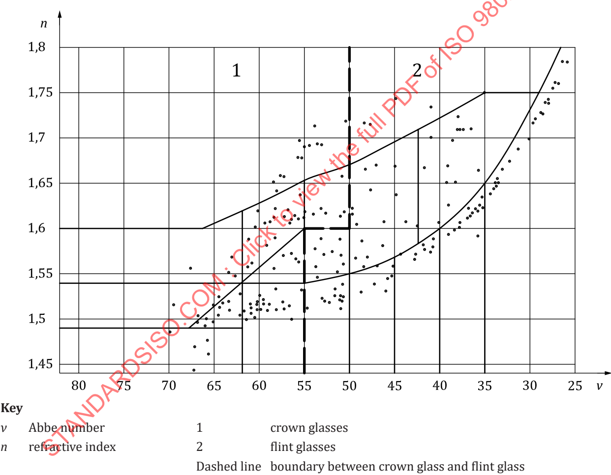
Figure 1 — Refractive index Abbe number diagram
