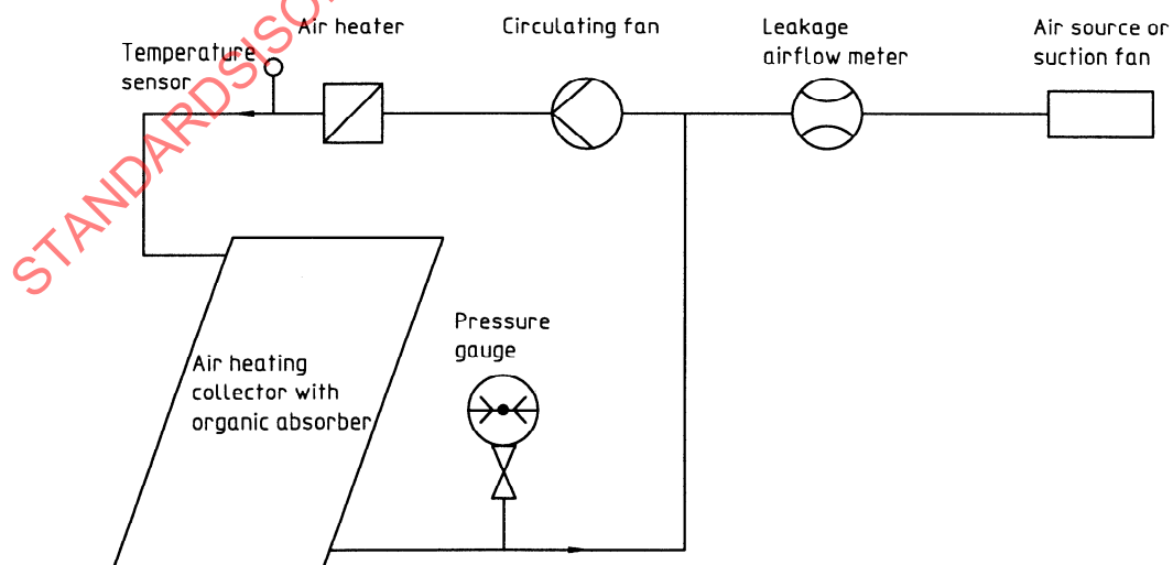
Figure 7 — Schematic for internal pressure test of air heating collectors with organic absorbers
