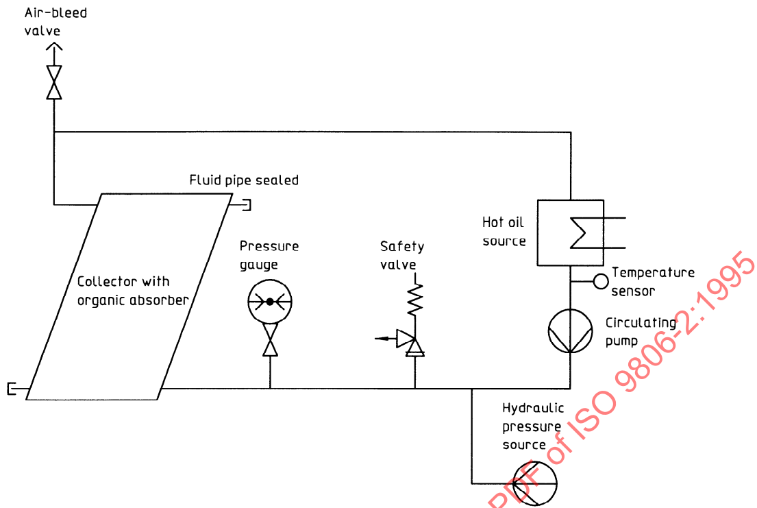
Figure 3 — Schematic for internal pressure test of organic absorbers for use with oil-based fluids (hot oil source)
