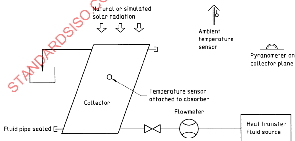
Figure 11 — Schematic for internal thermal shock test for liquid heating collectors
