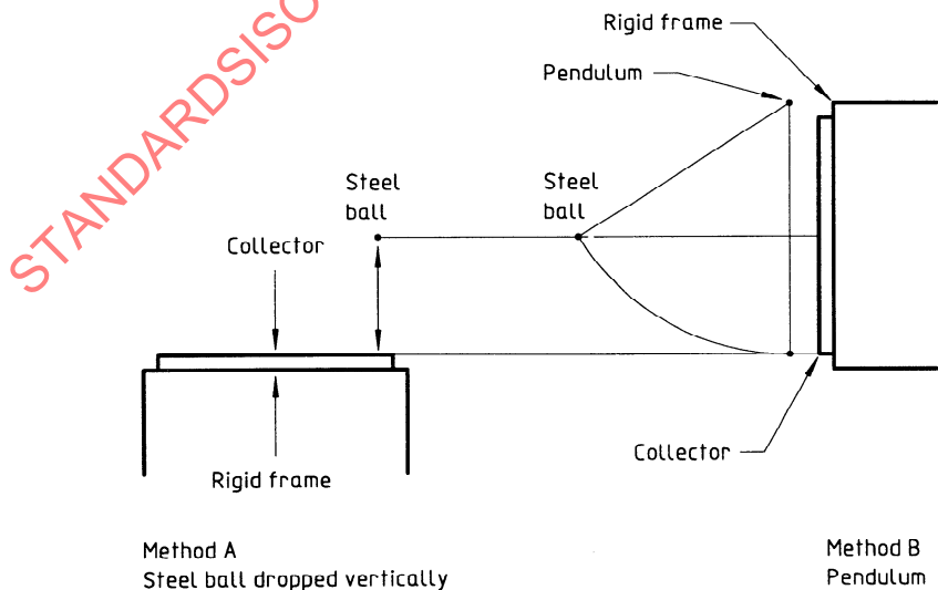
Figure 14 — Schematic for impact resistance test
