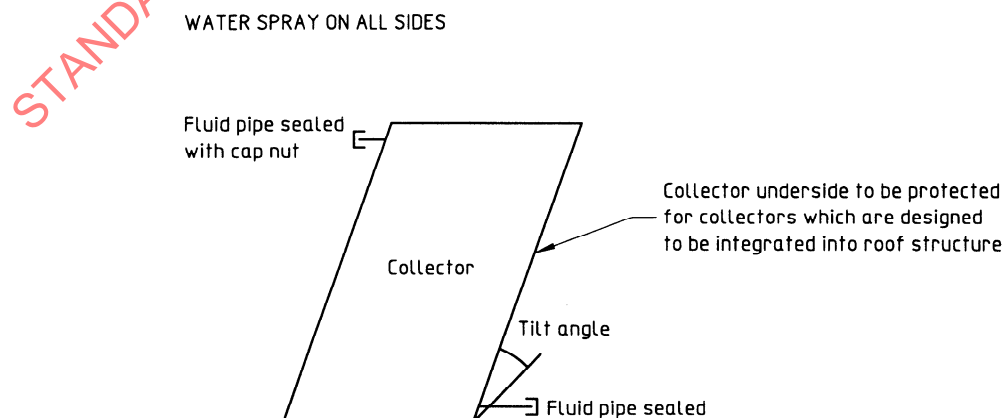
Figure 12 — Schematic for rain penetration test
