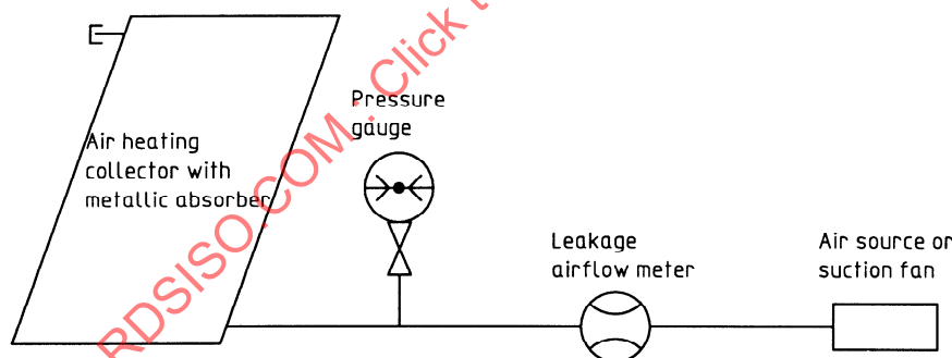
Figure 6 — Schematic for internal pressure test of air heating collectors with metallic absorbers
