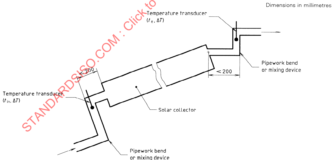
Figure 1 — Recommended transducer positions for measuring the heat transfer fluid inlet and outlet temperatures
