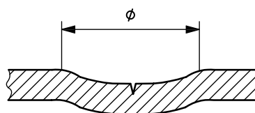
Figure A.2 — Dent containing cut or gouge
