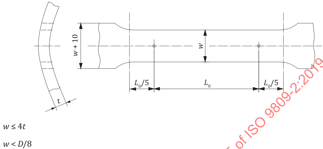
Figure 8 — Tensile test piece
