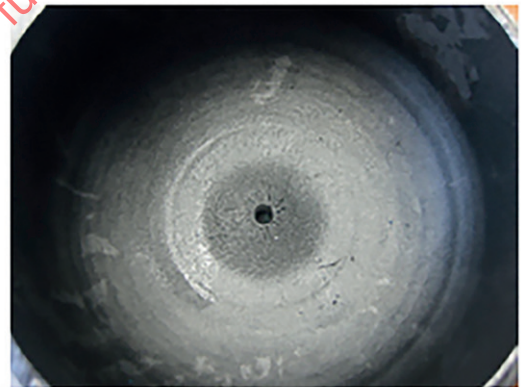
Figure A.11 — Features on cylinder base made from tube
