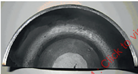
Figure A.10 — Examples of shoulder folds
