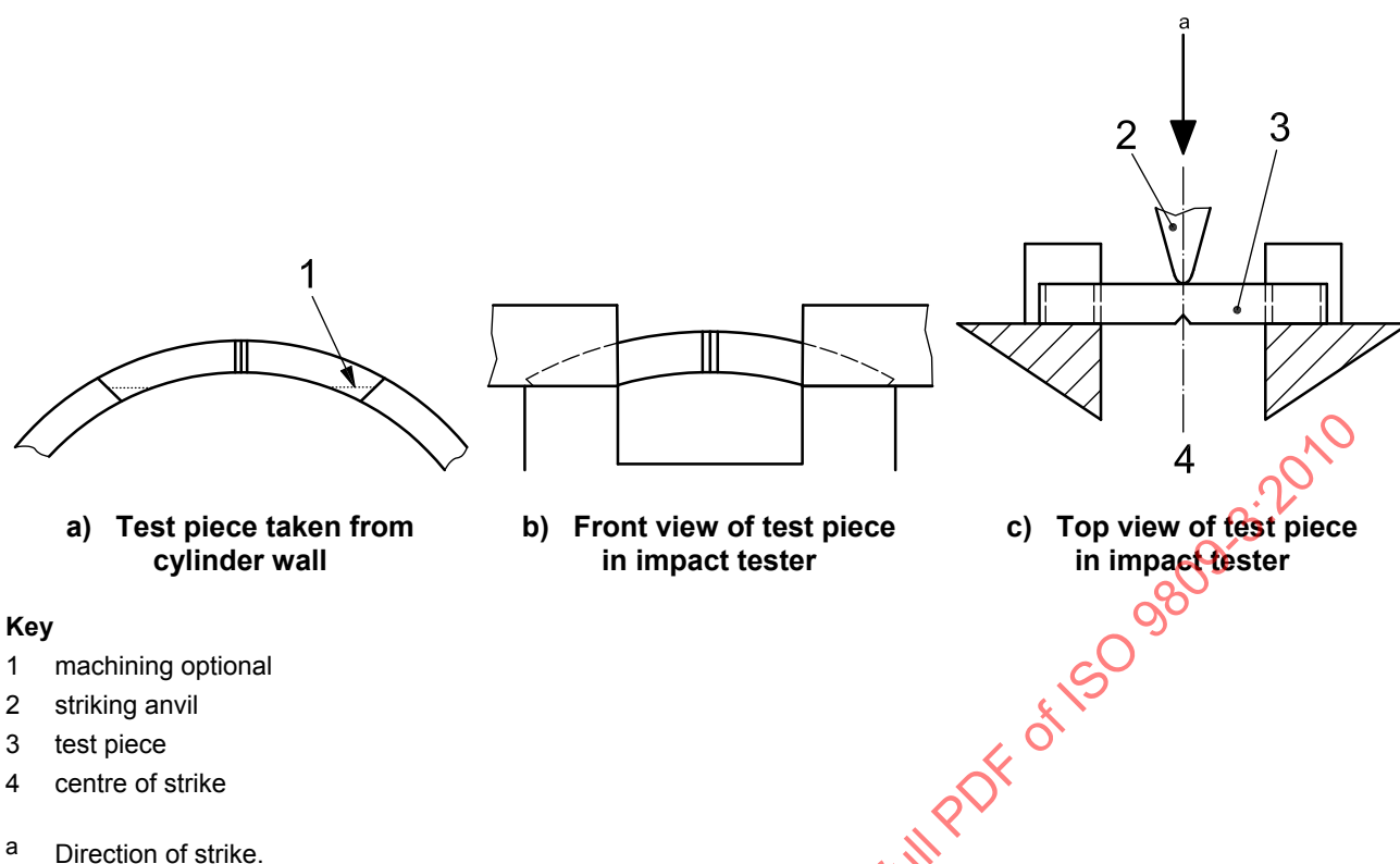
Figure 10 — Description of transverse impact testing
