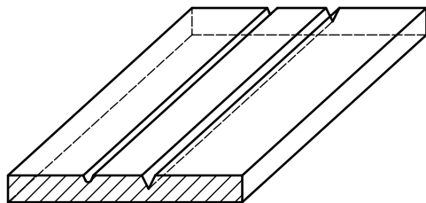
Figure A.4 — Dent containing cut or gouge
