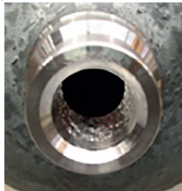
Figure A.13 — Chipped threads
