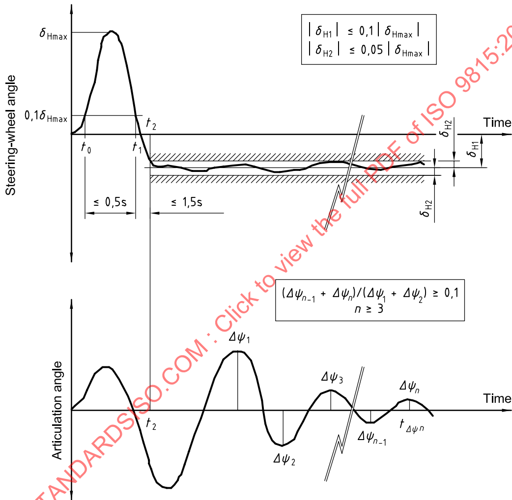
Figure 1 — Time histories of steering-wheel and articulation angles — Type 1
