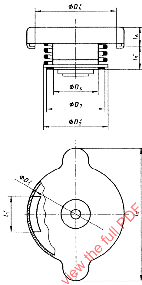
Figure 2 — Pressure cap
