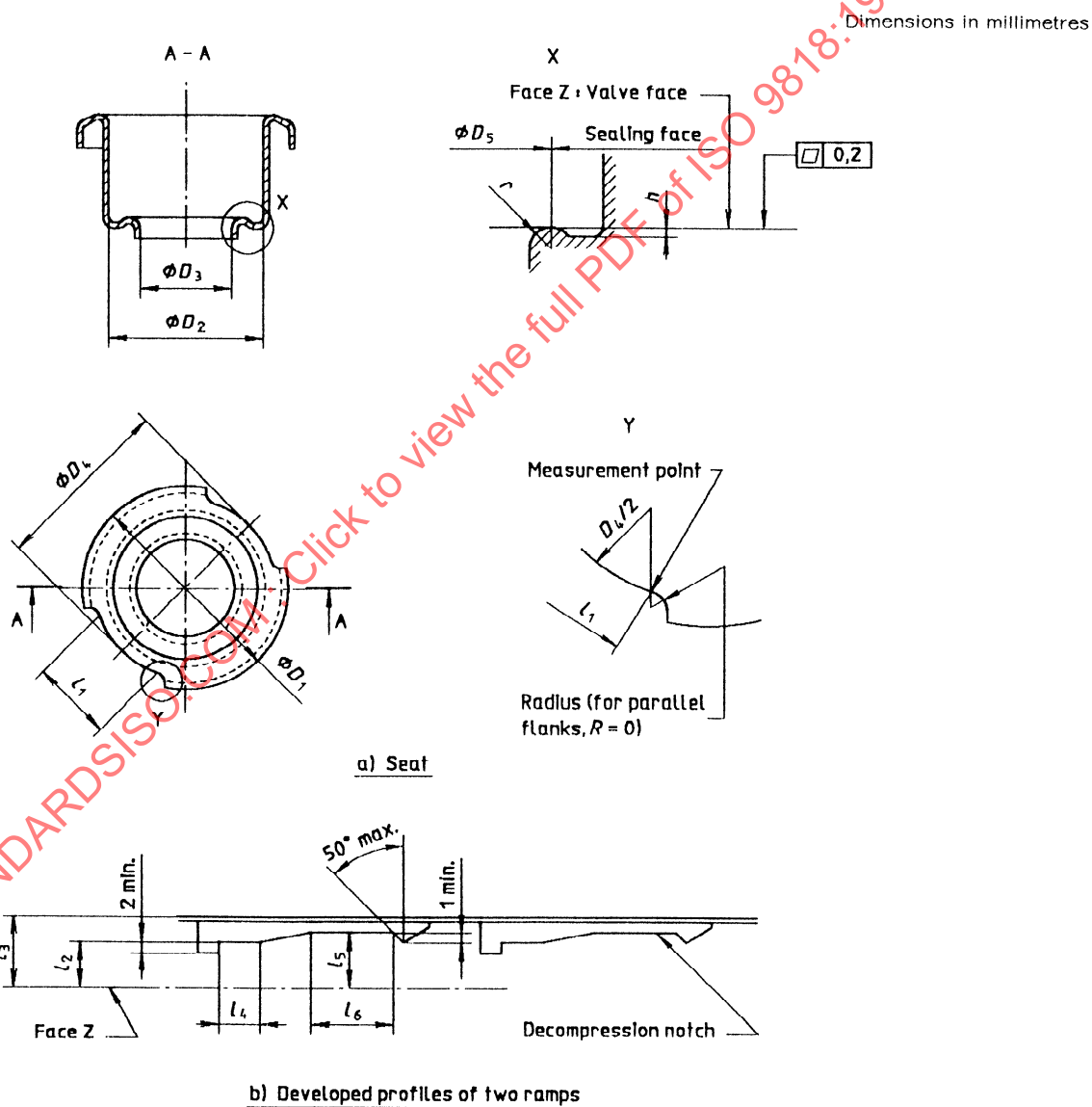
Figure A.1 — Seat with clamping ramps
