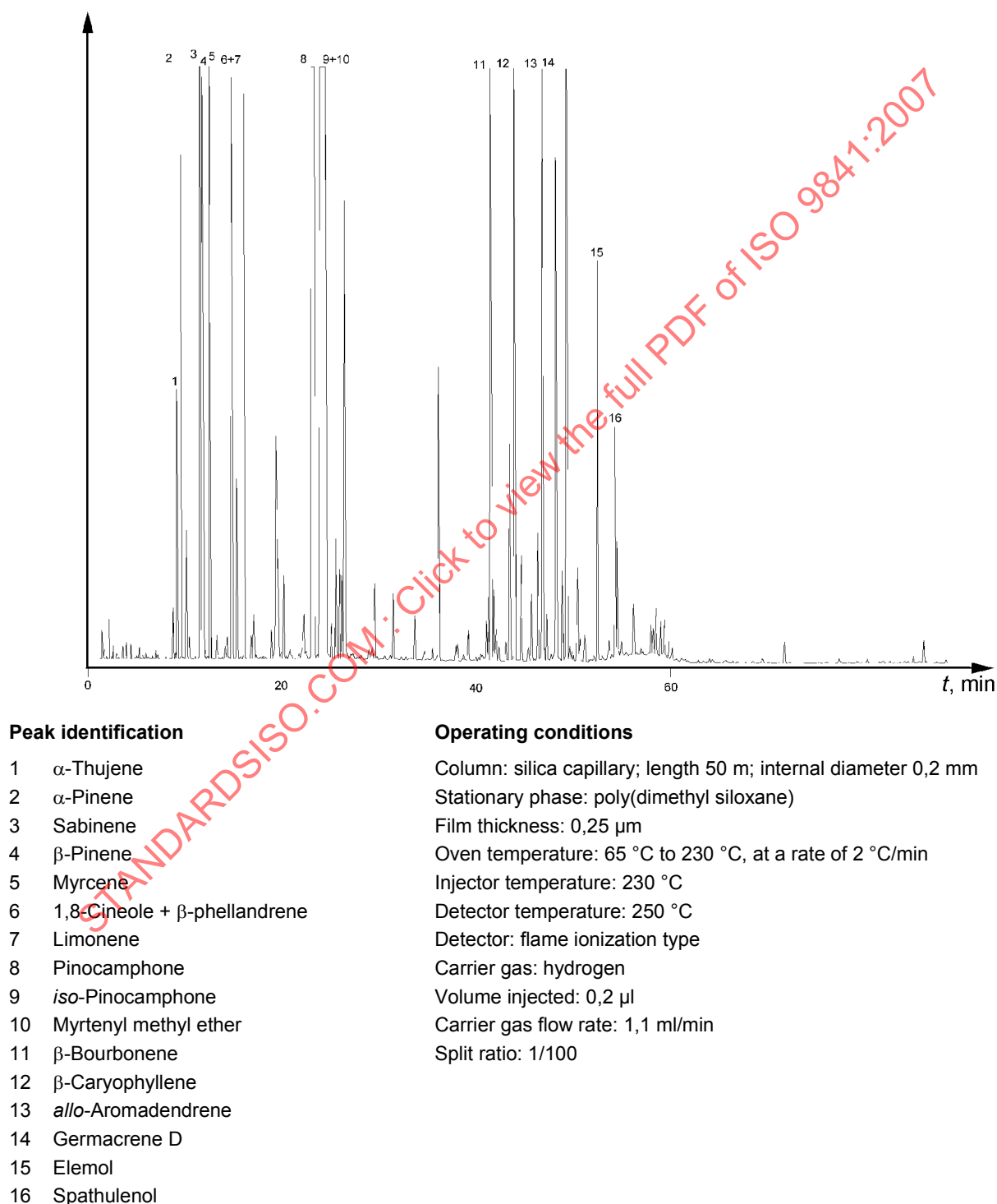
Figure A.1 — Typical chromatogram of oil of hyssop taken on an apolar column
