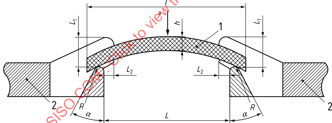
Figure 2 — Supports for specimen type 2 and type 3
