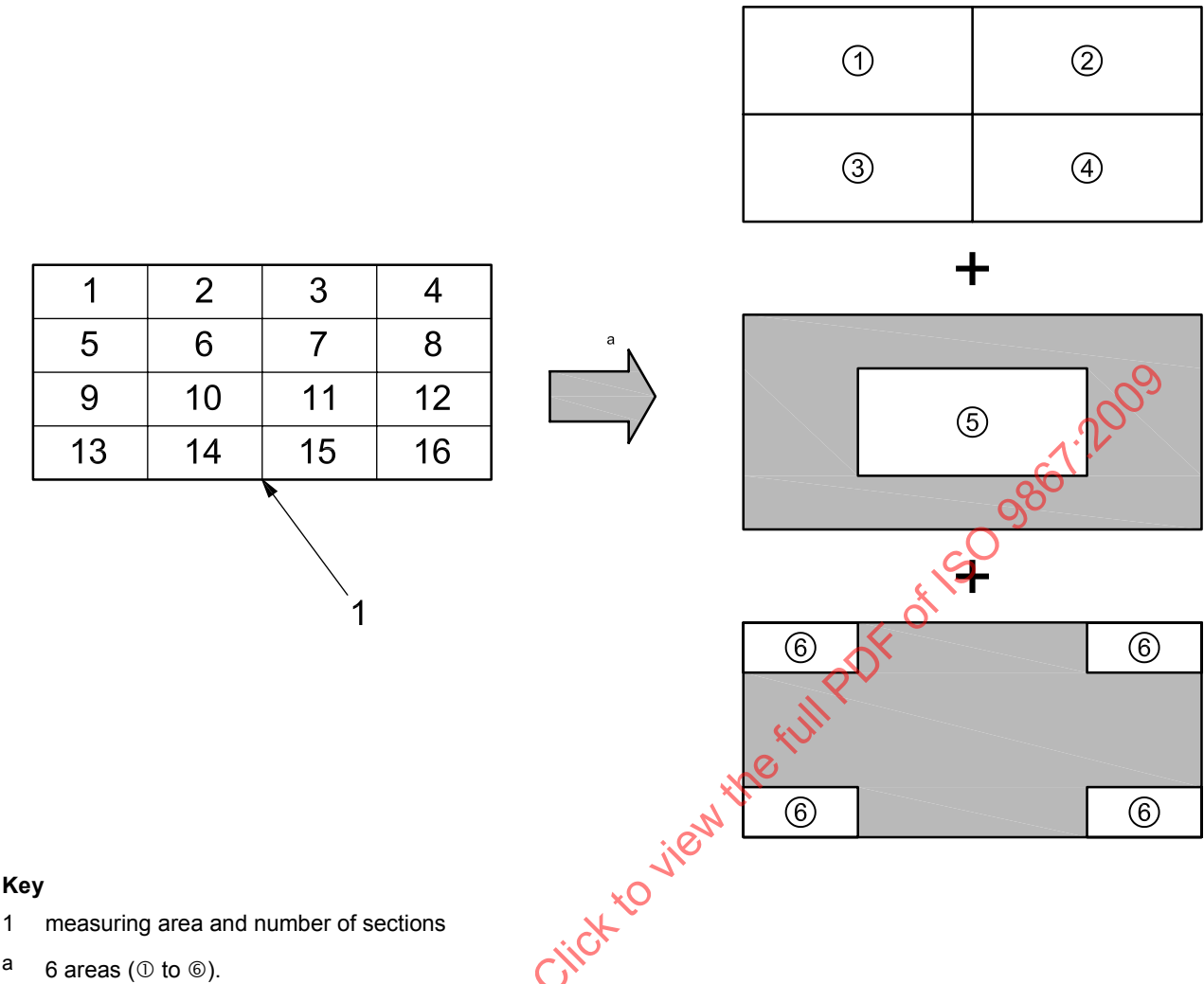
Figure B.3 — Six regions for wrinkle replica analysis
