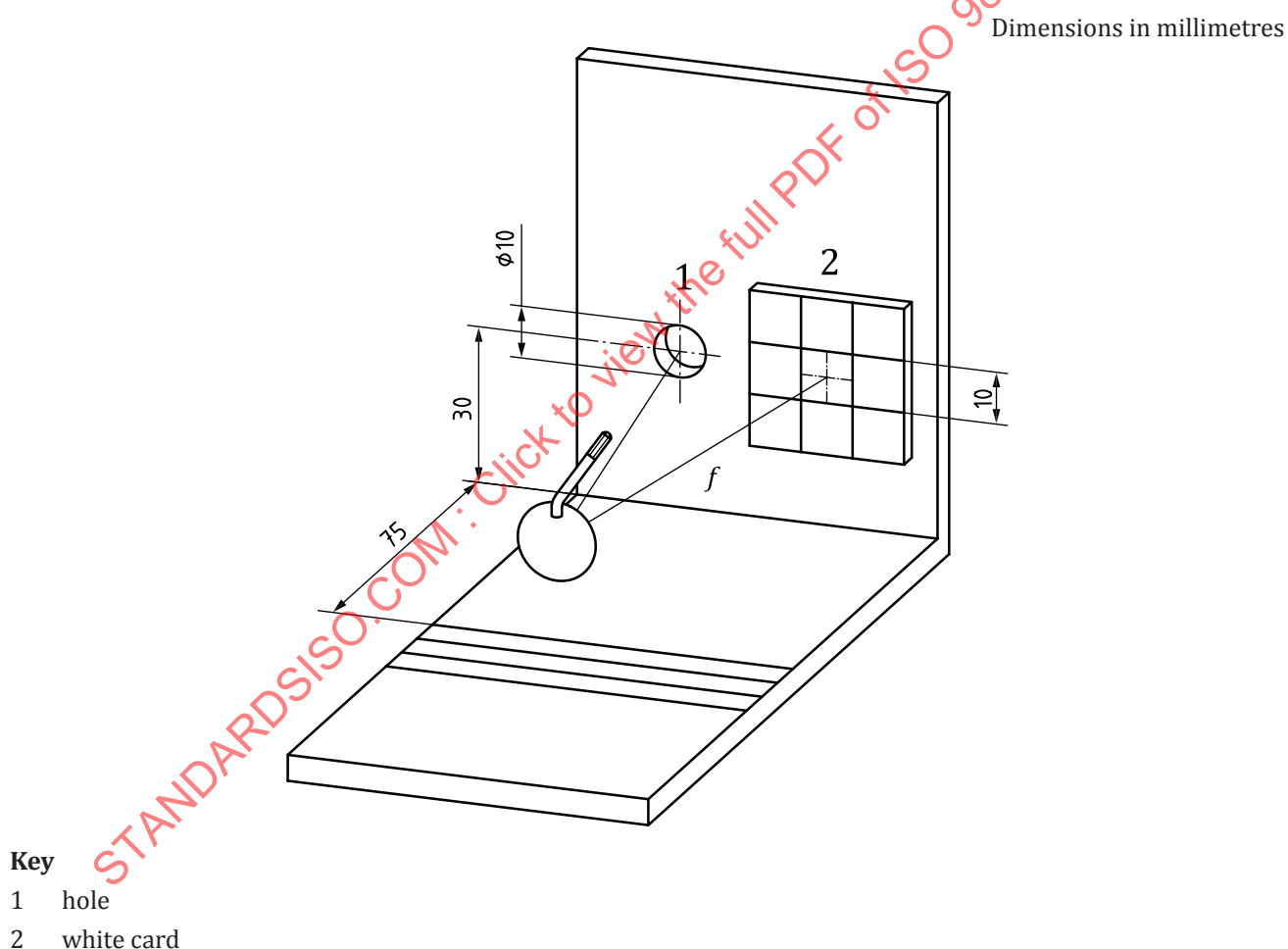
Figure 4 — Apparatus for determination of nominal magnification
