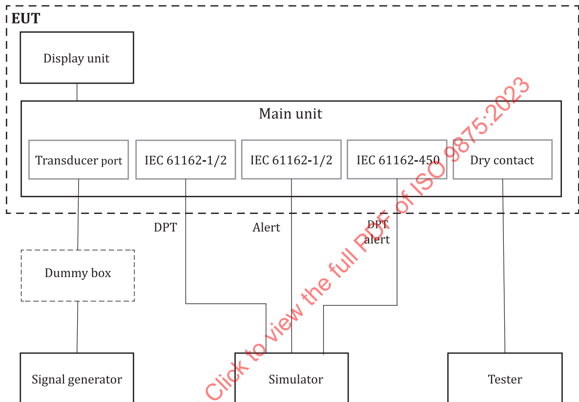
Figure 1 — Example of EUT and test configuration
