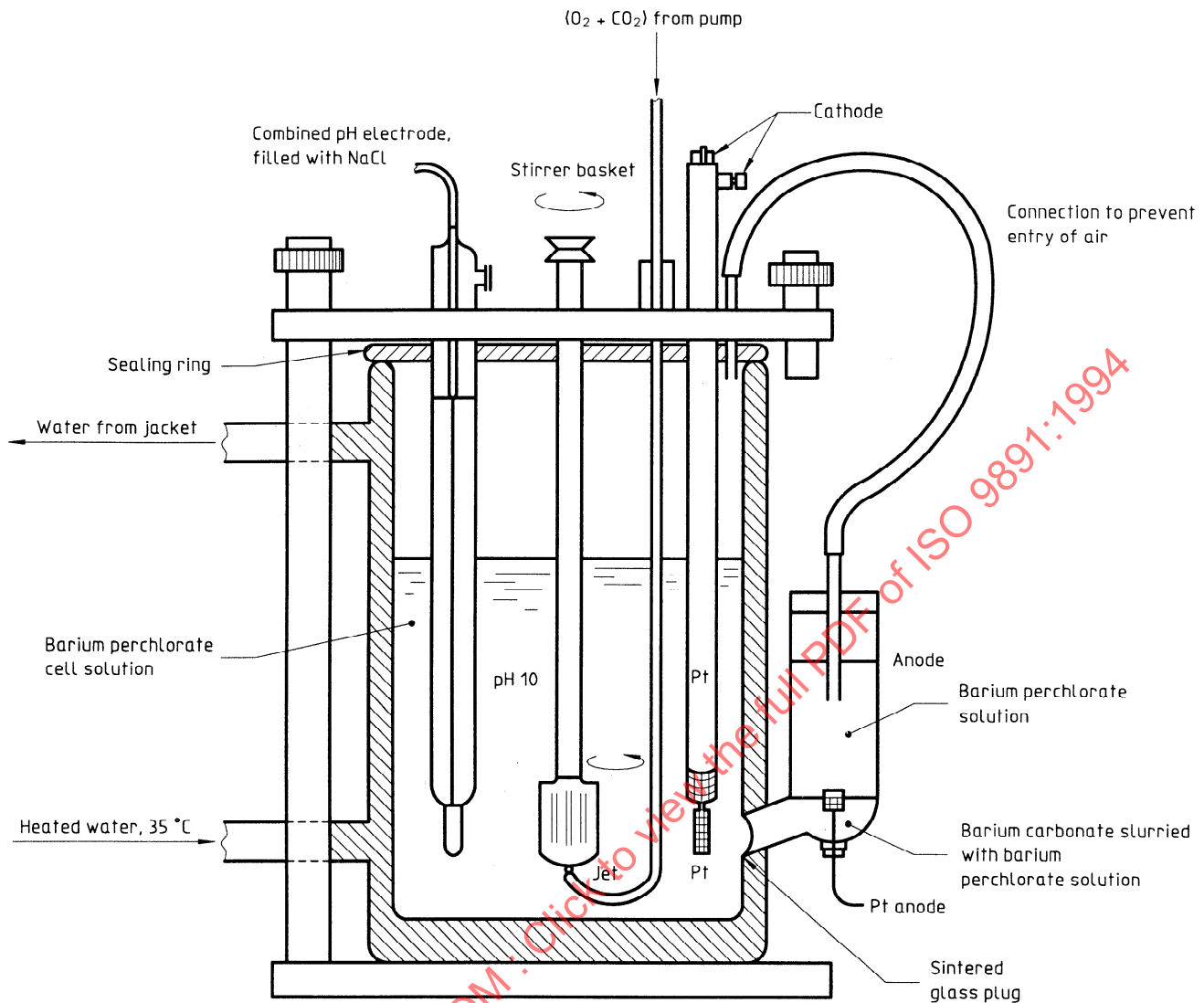
Figure 6 — Coulometric cell
