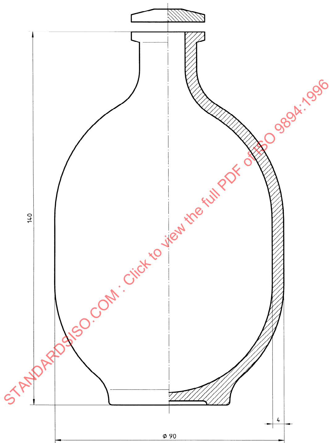
Figure 1 — Example of a PTFCE container (0,5 litre) for chemical analysis
