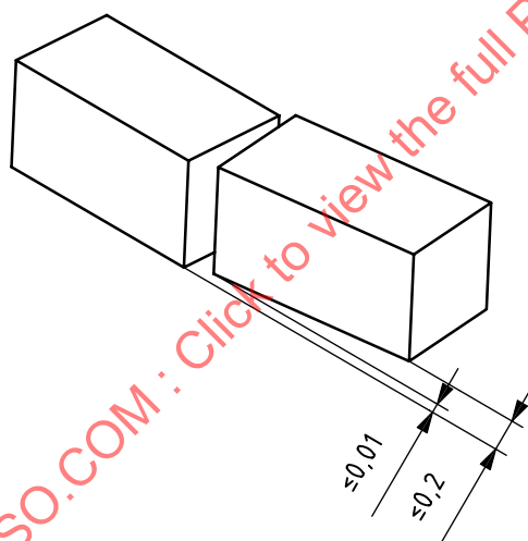
Figure A.1 — Specifications for the maximum permissible departure from parallelism of the clamping surfaces
