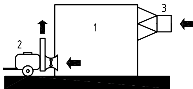
a) Set-up for a one way sucking air-assisted sprayer in the measuring chamber
