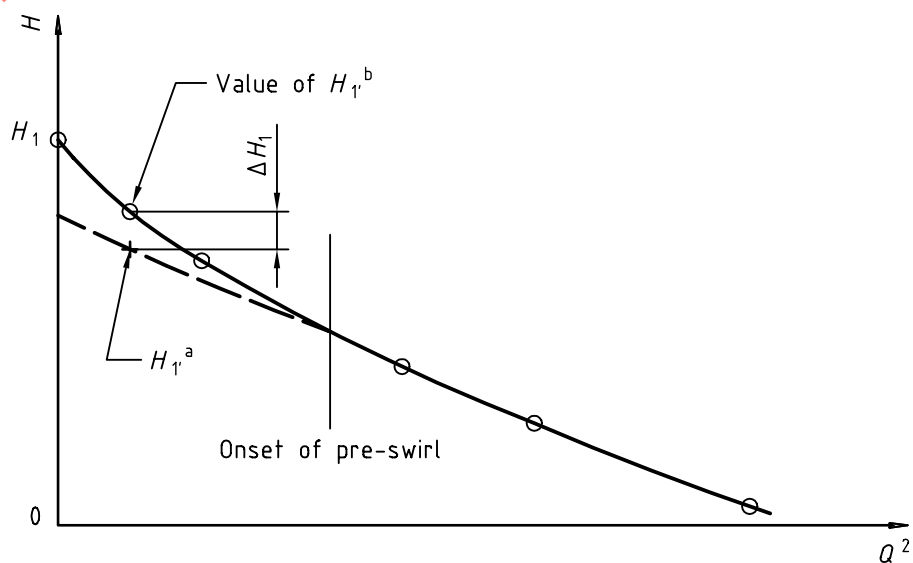
Figure 5 — Correction of inlet total head
