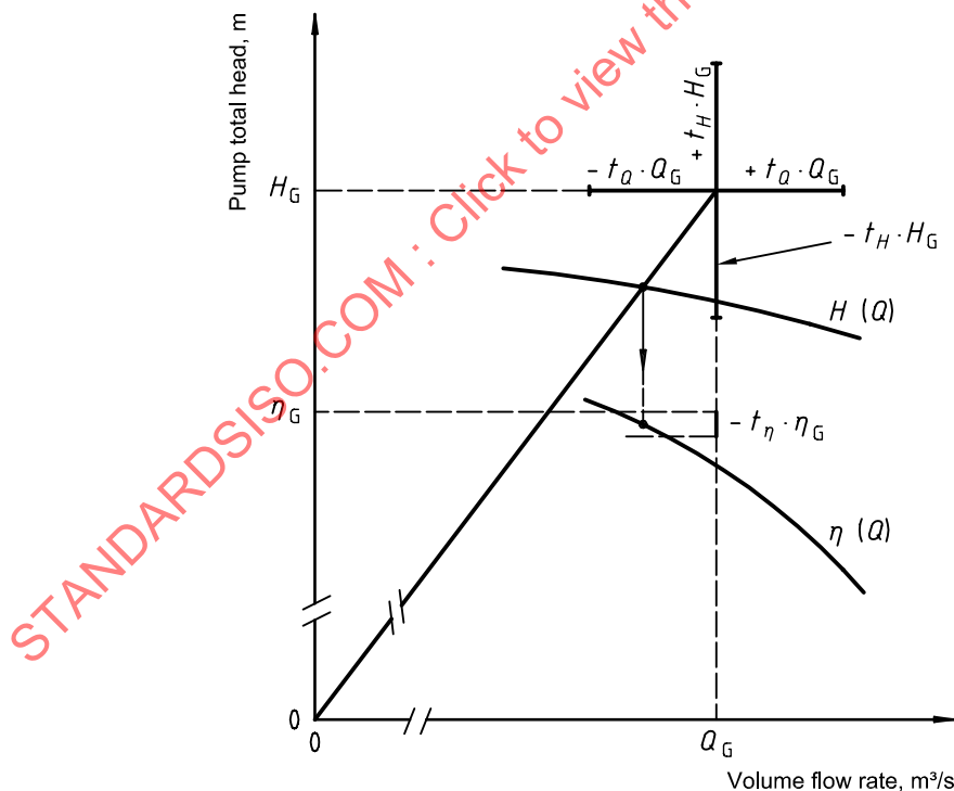
Figure 2 — Verification of guarantee on flow rate, head and efficiency
