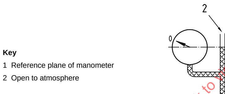
Figure 11 — Arrangement for determination of reference plane of spring pressure gauges
