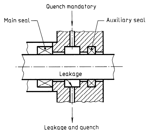
Q3 Main seal with auxiliary seal or packing
