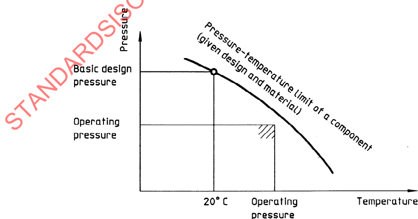
Figure 1 — Relationship between temperature and pressure
