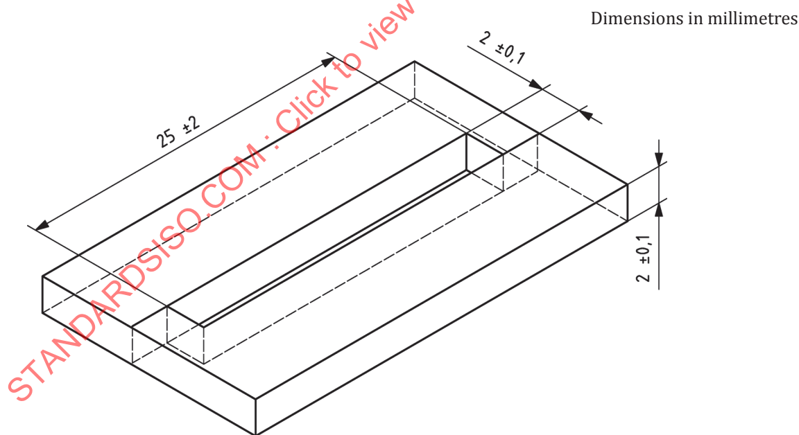
Figure C.1 — Mould for flexural strength specimen
