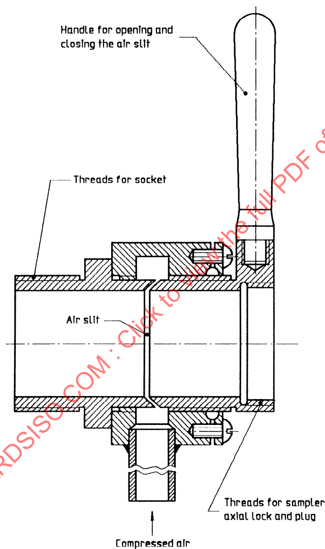
Figure A.2 — Dustless connection
