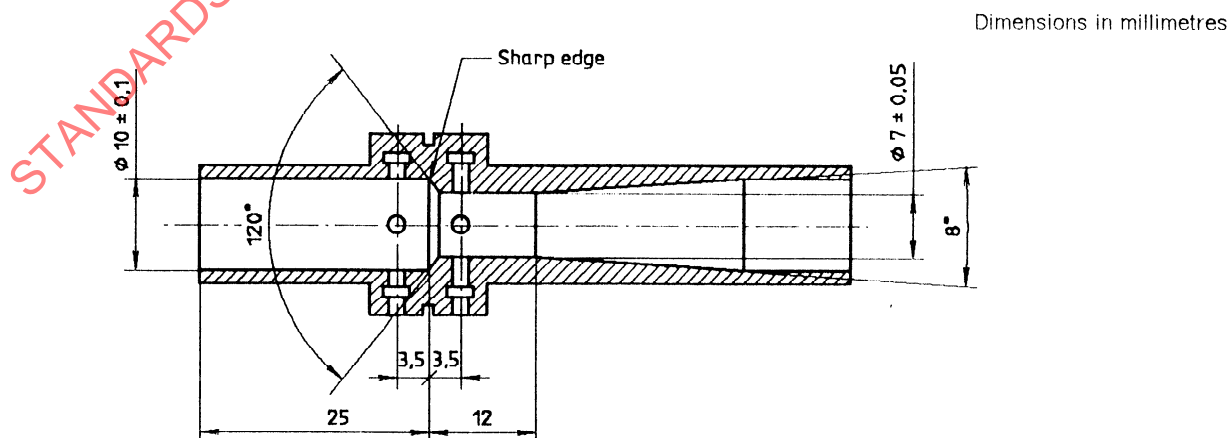
Figure A.6 — Example of a suitable Venturi nozzle
