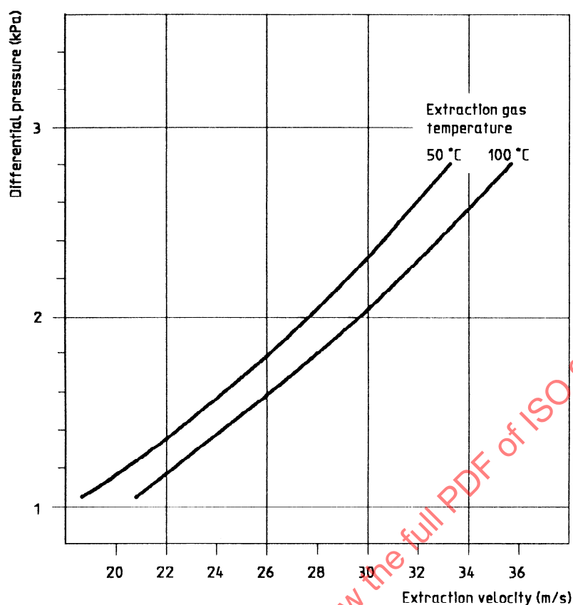
Figure A.7 — Calibration chart for the Venturi nozzle shown in figure A.6
