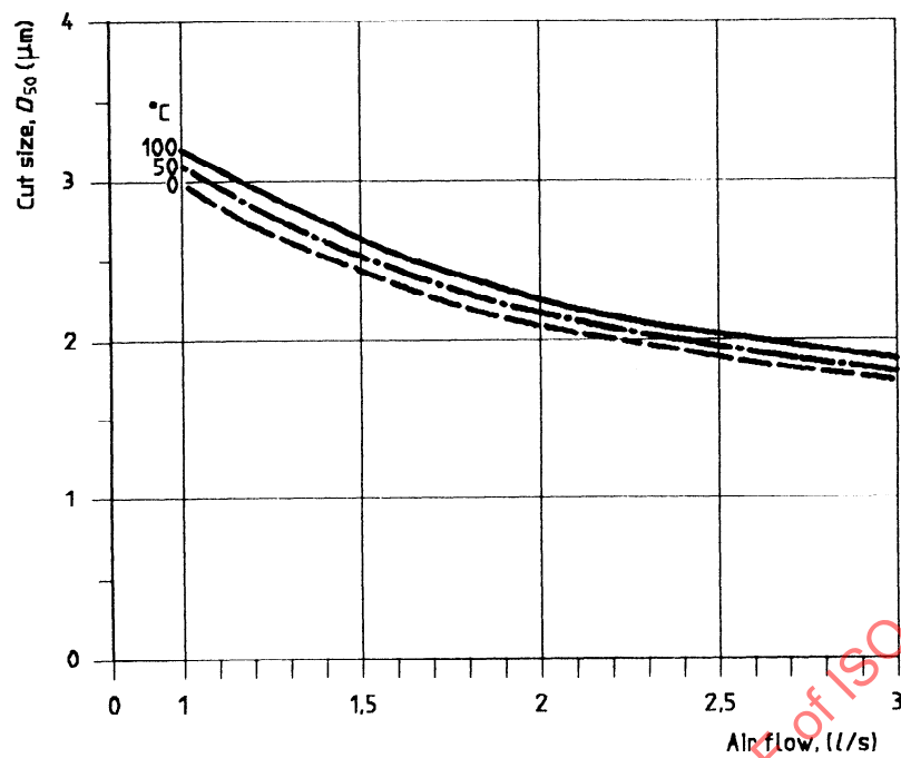
Figure A.4 — Cut size ( D_{50} ) for cyclone in figure A.5
