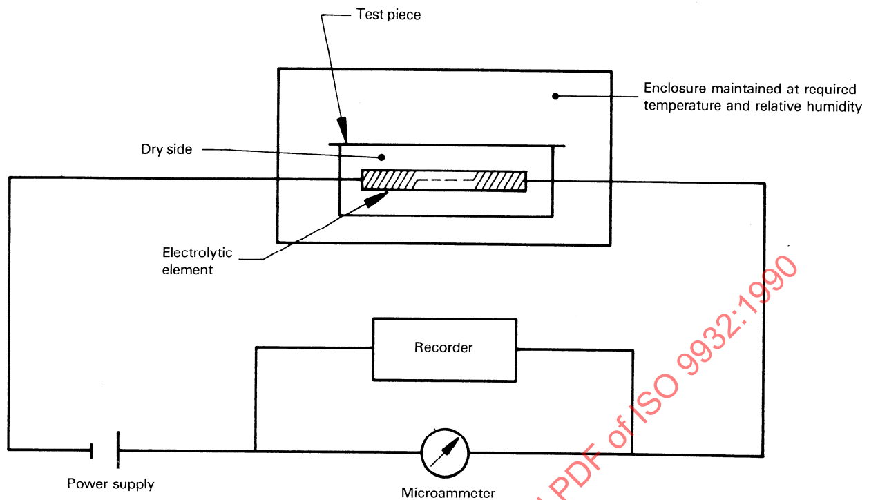
Figure 2 — Schematic diagram of static system
