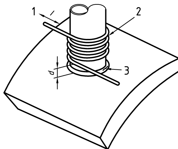
Figure 5 - Threading conductor
