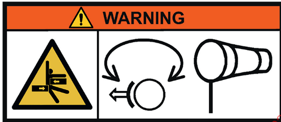
Figure A.7 — Example of a safety label: shearing hazard when slewing brake is unlocked to allow weathervaning
