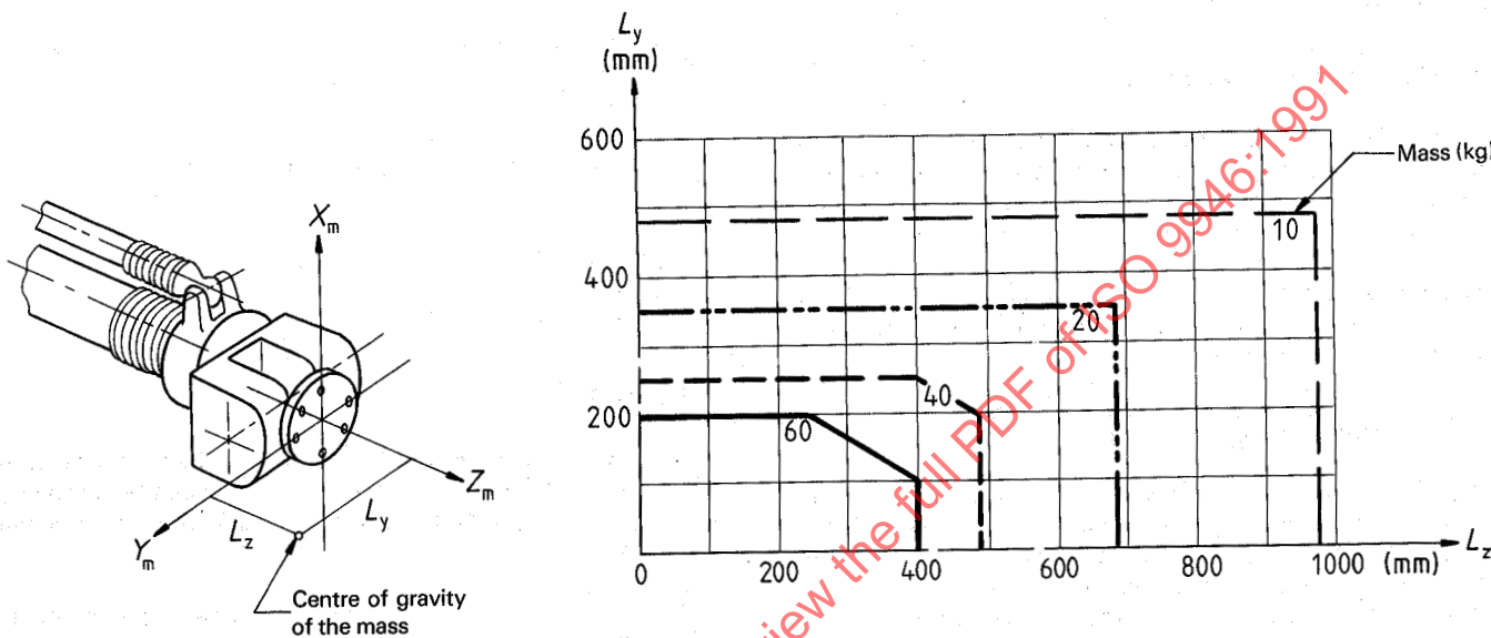
Figure 3 — Load diagram
