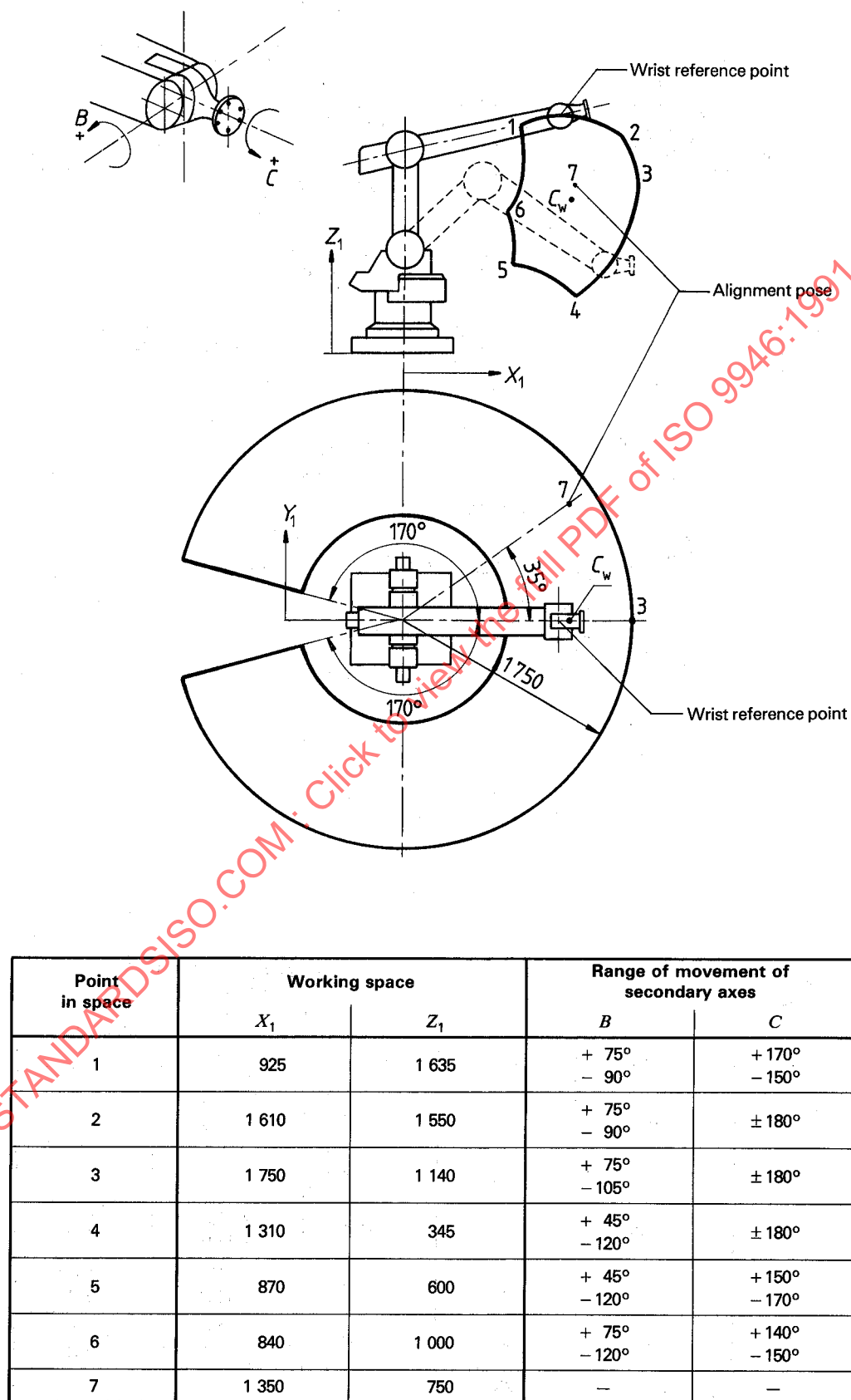
Figure 1 — Example of 5-axis robot working space
