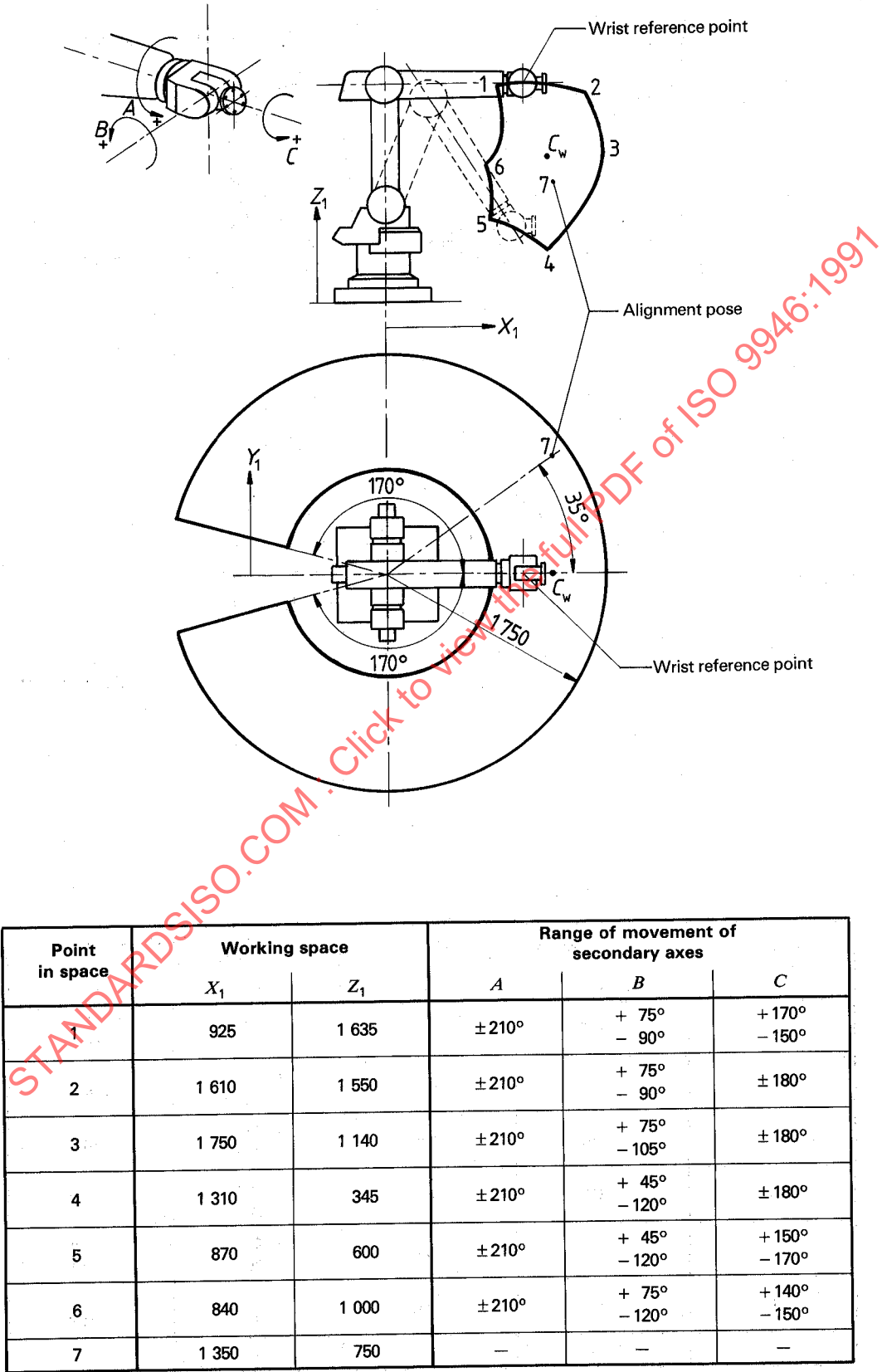
Figure 2 — Example of 6-axis robot working space
