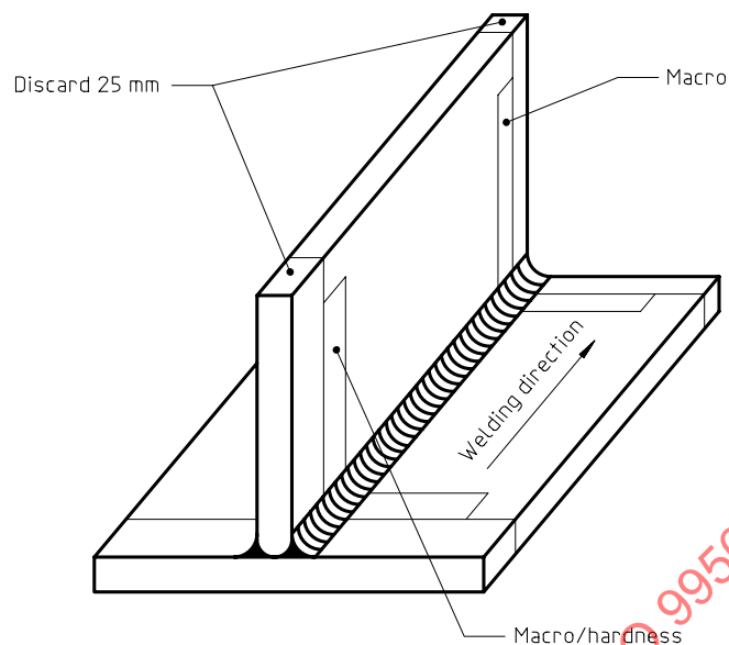
Figure 8 — Location of test specimens in a T-butt joint or a fillet weld on plate
