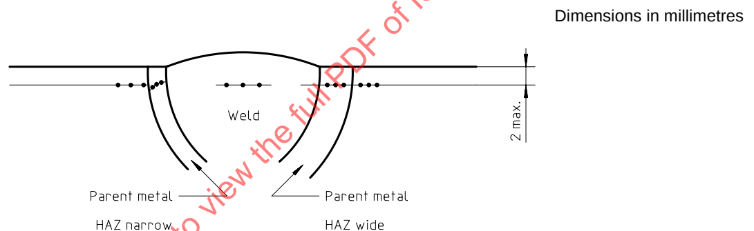
Figure 10 — Typical example of hardness testing
