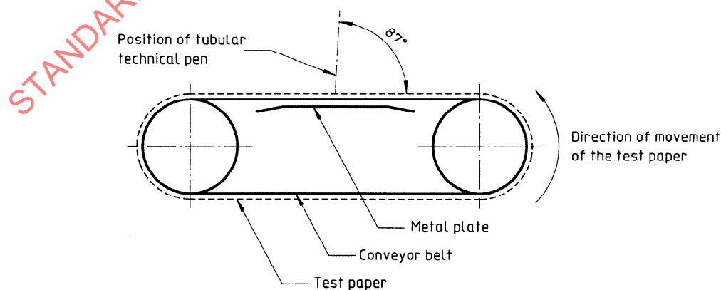
Figure 1 — Schematic representation of the test machine
